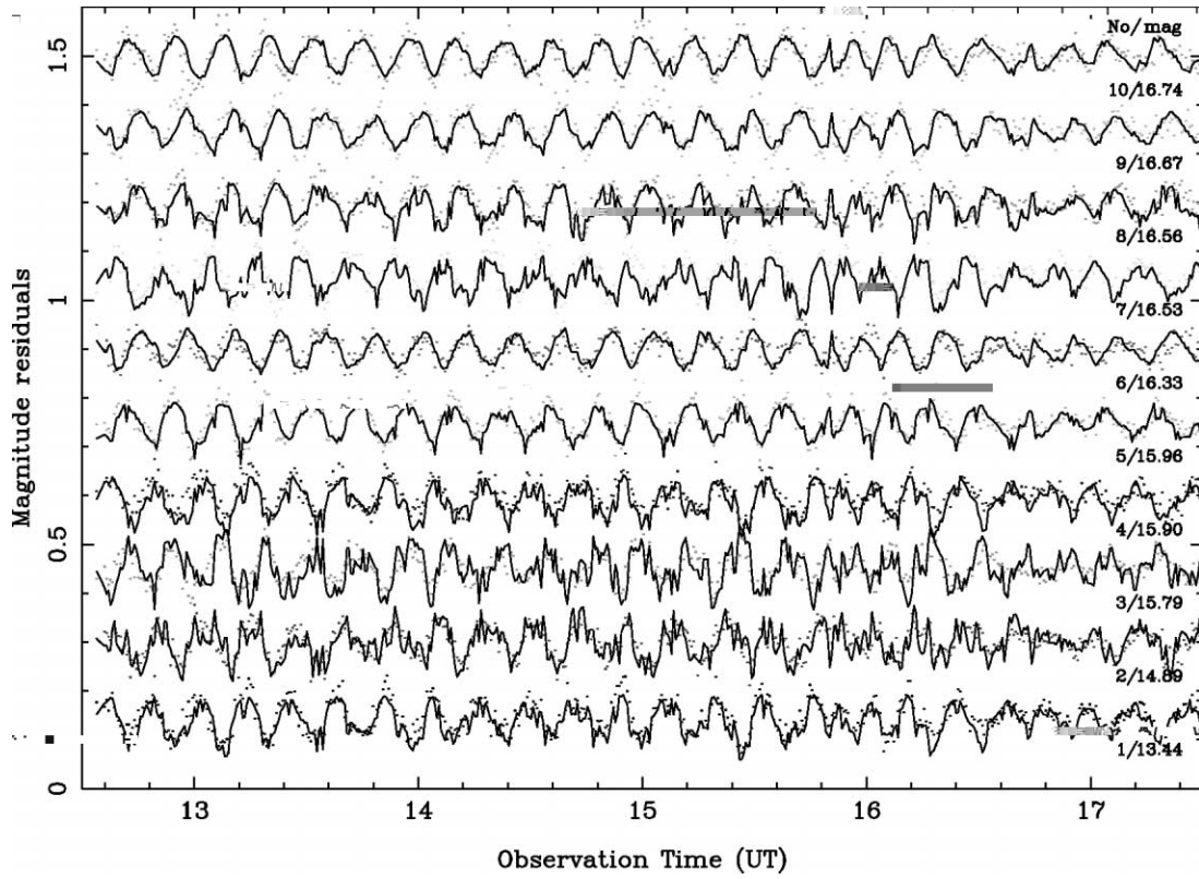
FIG. 5.—Residual light curves of the 10 brightest stars in the first 5 hr of observation on the night of 2003 November 23. The axis labels are the same as in Fig. 3. The solid lines represent the simulation, based on intrapixel position and seeing (see text).
