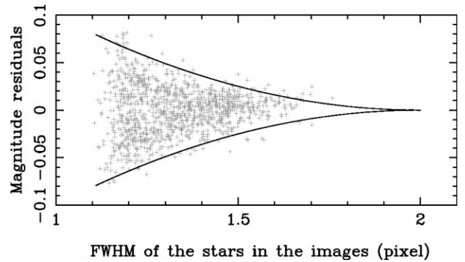
FIG. 8.—Magnitude variation vs. seeing of the image. The solid parabolic curves represent the magnitude residual as a function of seeing. A total of 20 bright stars were used to obtain this relation, but only the data points of the brightest star are shown.
