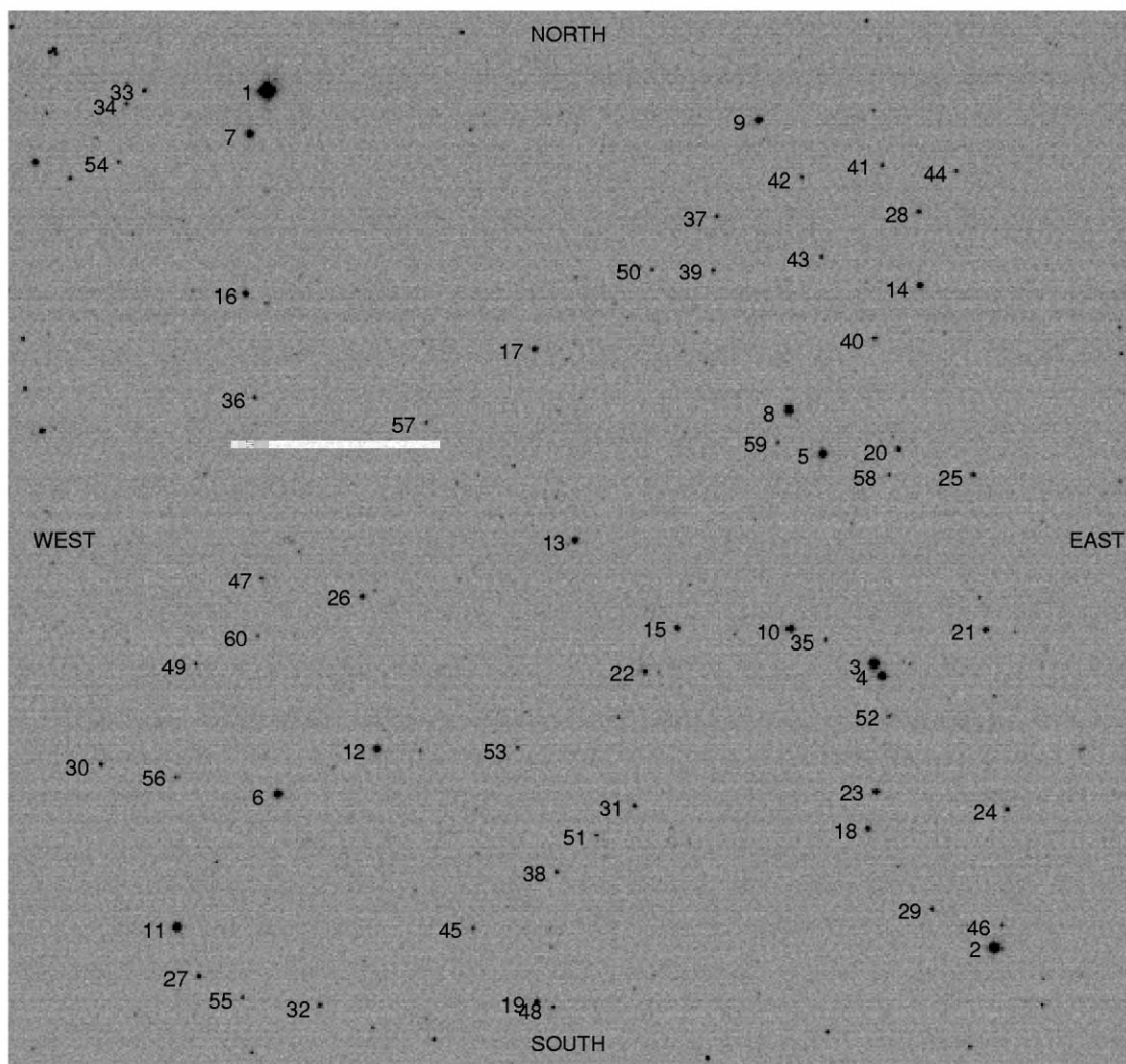
FIG. 1.—Reference frame image with a 14' \times 14' field of view. A total of 60 stars are identified and monitored for brightness variation in the 10 hr period.
