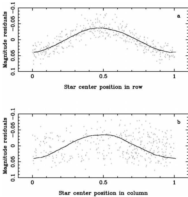
FIG. 7.—Variation of the observed magnitude vs. vertical subpixel position (a) and vs. horizontal subpixel position (b). The smoothed curve traces the variation due to the intrapixel effect. A total of 20 bright stars were used to obtain this correlation, but only the data points from the brightest stars are shown here. The change of residual is very obvious along the y -direction, but is not so clear along the x -direction. This may be a result of either the readout direction of the CCD or the tracking error in R.A.
