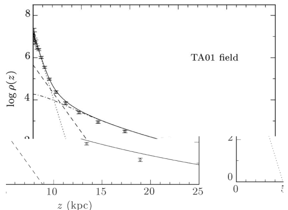
Fig. 4. As Fig. 3, but the density distribution are plotted for the TA01 field.
