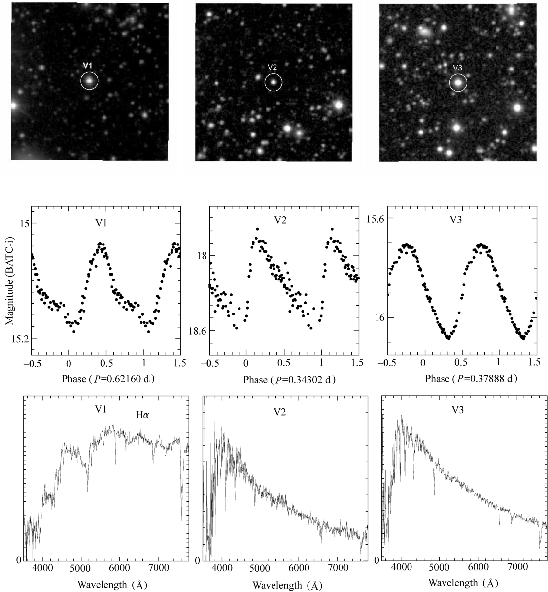
Fig. 1 Finding charts, phased light curves and spectra of three new variables. The circles in the finding charts have radius 10 arcsec.
