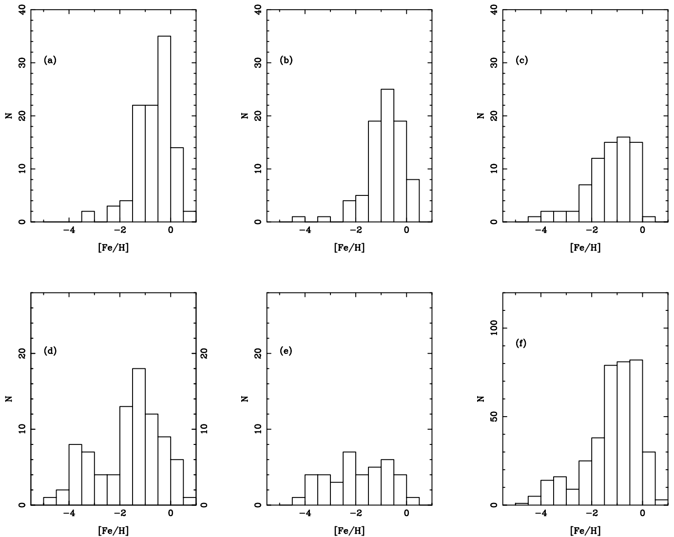
FIG. 7.—Metallicity distribution for sample stars as functions of apparent magnitude i . (a) 14.0 < i \leq 15.5 , (b) 15.5 < i \leq 16.5 , (c) 16.5 < i \leq 17.5 , (d) 17.5 < i \leq 18.5 , (e) i > 18.5 , and (f) 14.0 < i \leq 20.5 .
