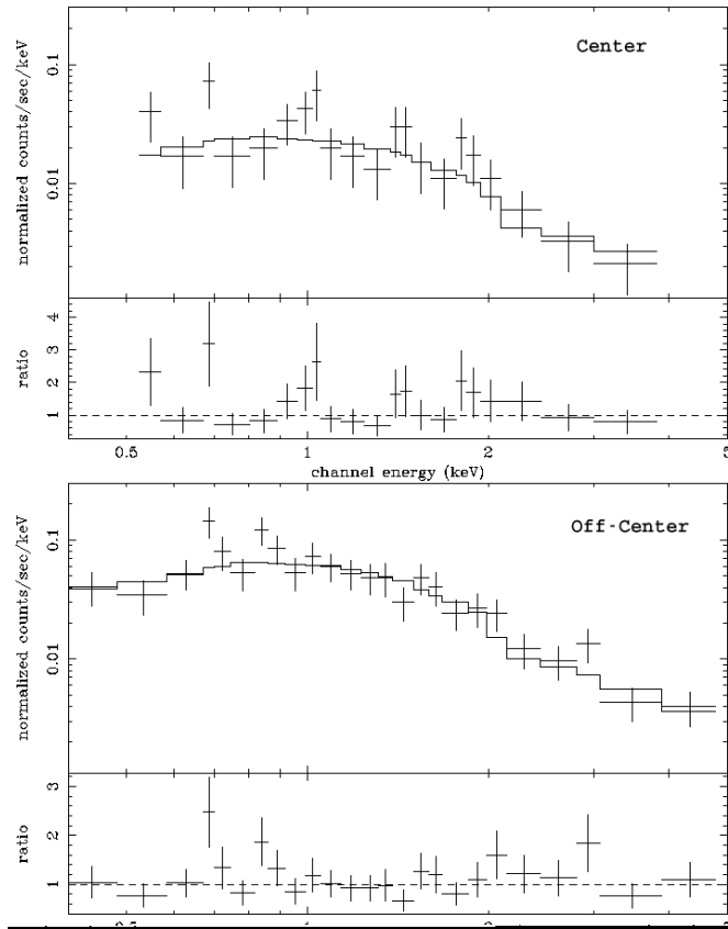
FIG. 2.—X-ray spectra for the nuclear source RX J1236.3+2559 ( top panel ) and the off-center source RX J1236.2+2558 ( bottom panel ) in NGC 4565. The spectrum of the nuclear source is fitted by an absorbed power law, and the off-nucleus source is fitted by an absorbed multicolor disk model. The fitting parameters are listed in Table 2.
