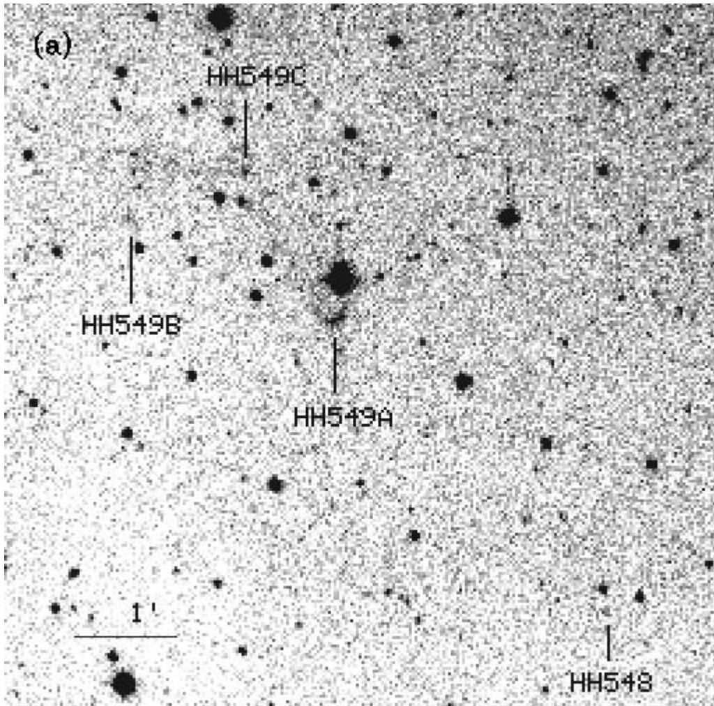
FIG. 1.—[S II] images of the newly discovered HH objects: (a) HH 548 and 549A–C, (b) HH 550 and 551, (c) HH 552, and ( ) HH 553A–E and 554. North is up, and east is left.
